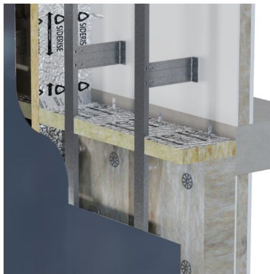
Horizontal cavity barrier in external wall – Image courtesy of Siderise Ltd
