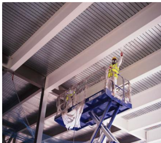
Fire resisting floor supported on a steel frame
